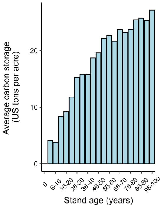
Carbon storage in MO
