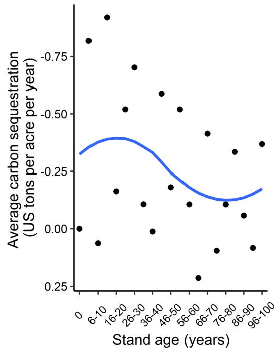
Carbon sequestration in MO
