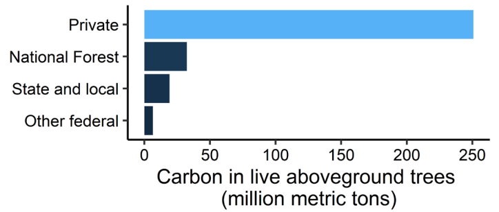
Carbon pools in MO forests
