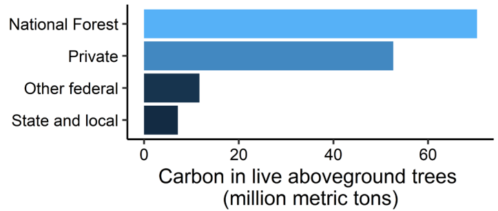
Carbon pools in AZ forests
