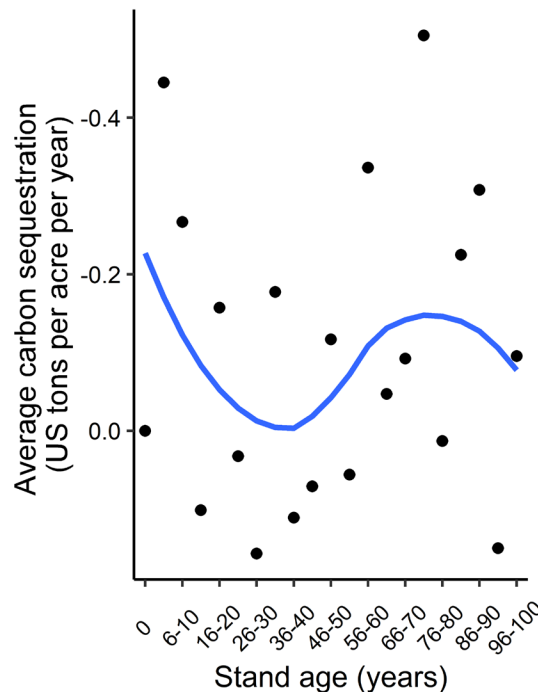
Carbon sequestration in AZ
