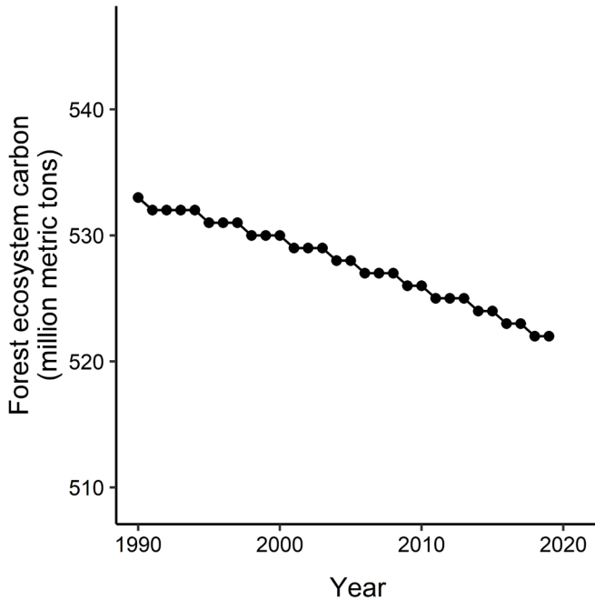
Trends in Arizona
