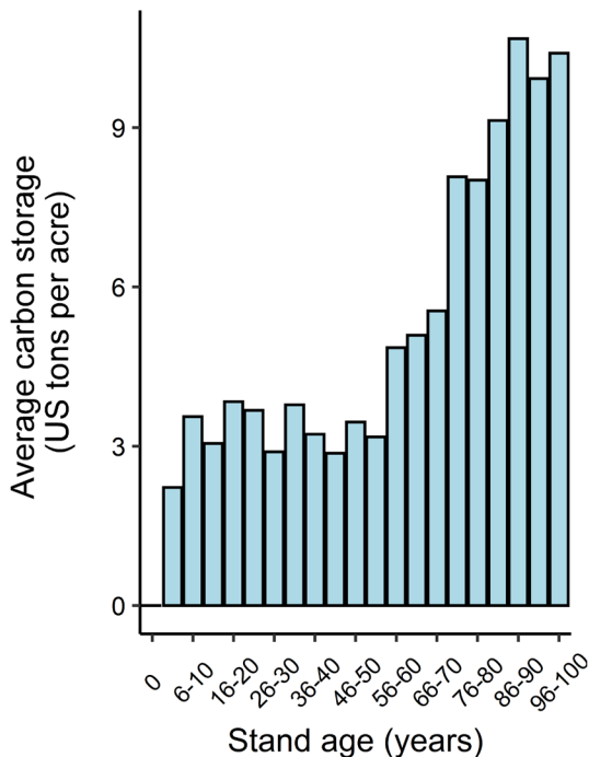
Carbon storage in AZ
