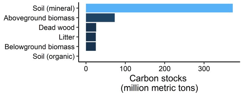
Carbon sequestration in AZ
